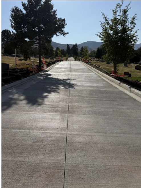
Completed pavement on 1100E
