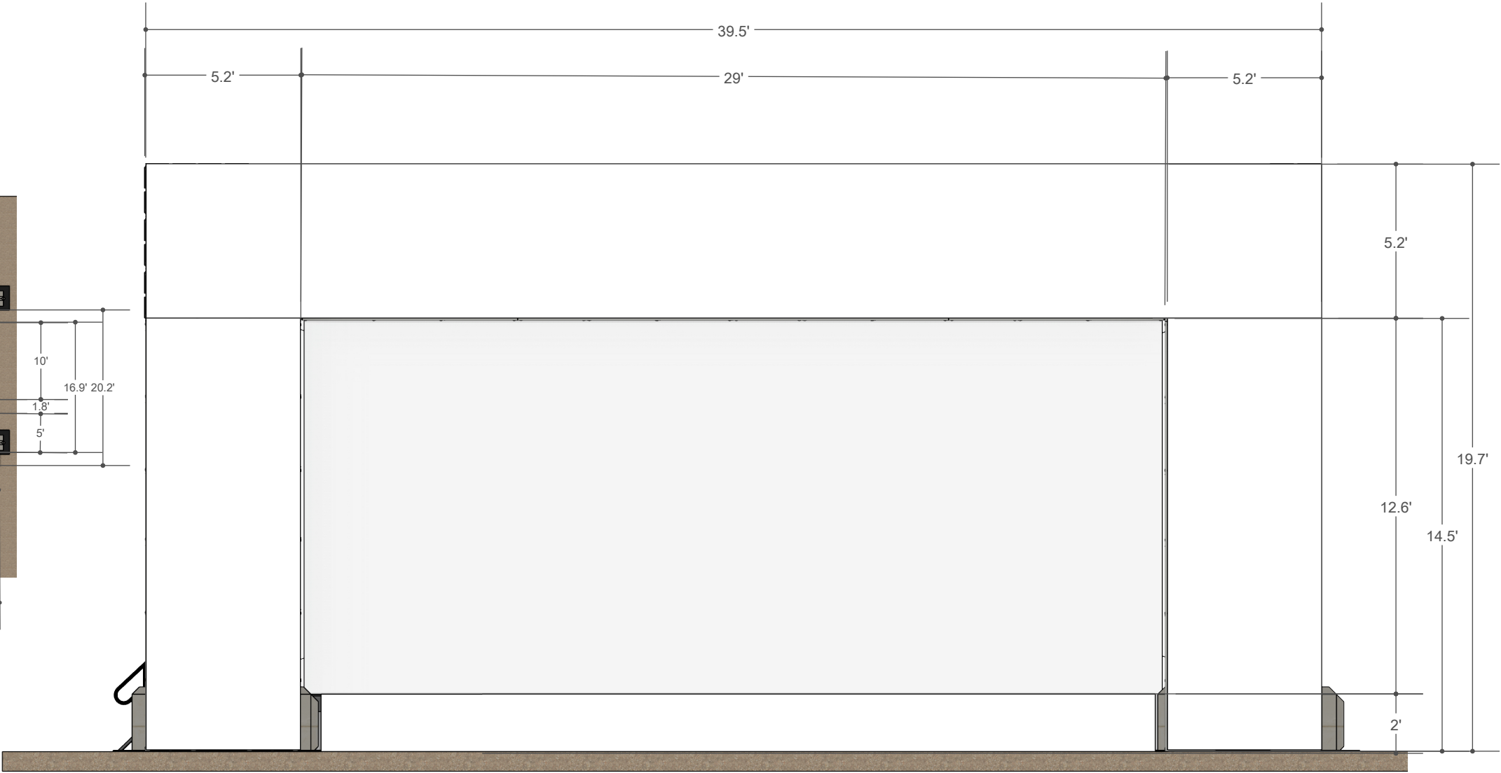
FRONT VIEW
