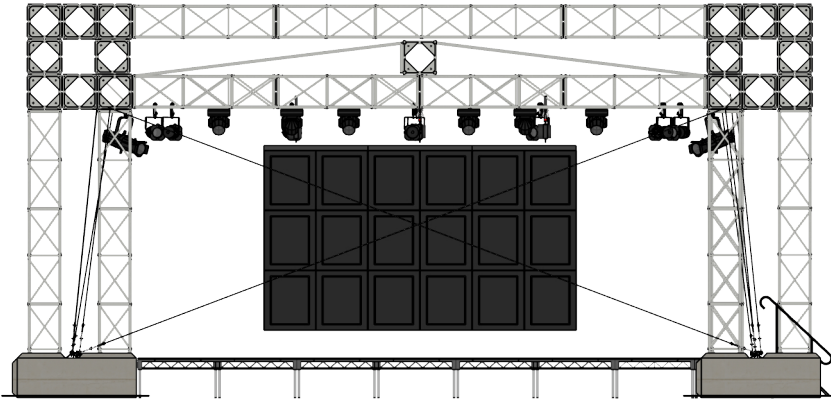
OVERHEAD PROFILE
