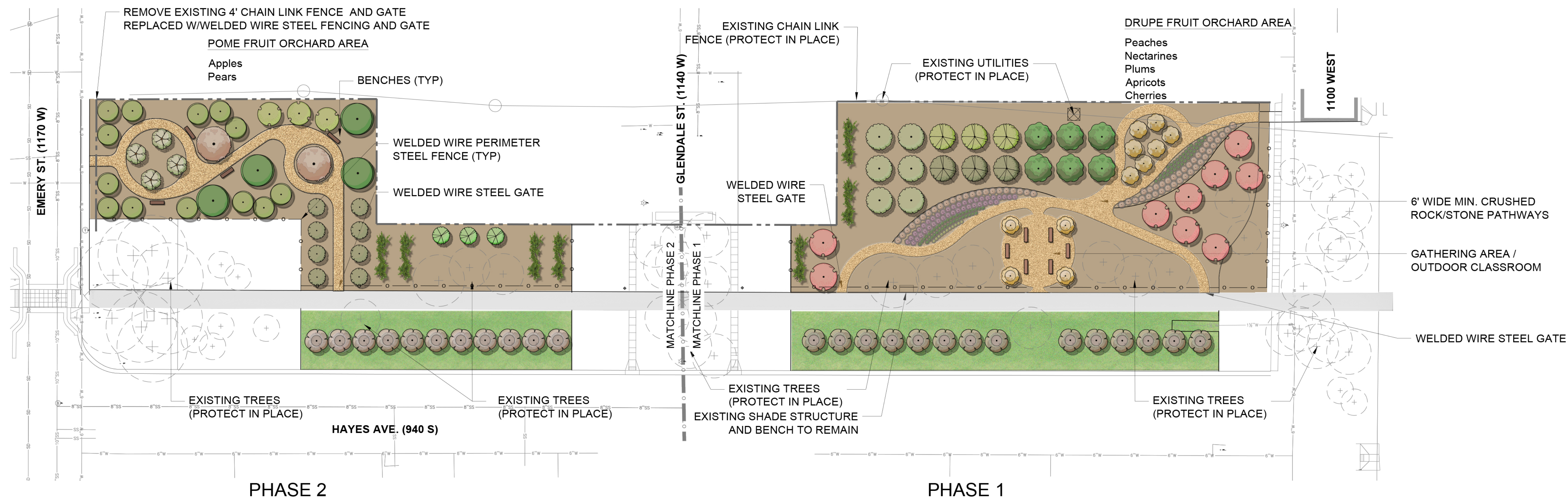
1 OVERALL LANDSCAPE PLAN 1" = 30'-0"
