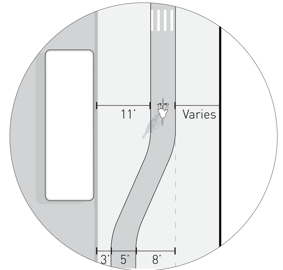
Type C Bus Stop Island - Large
